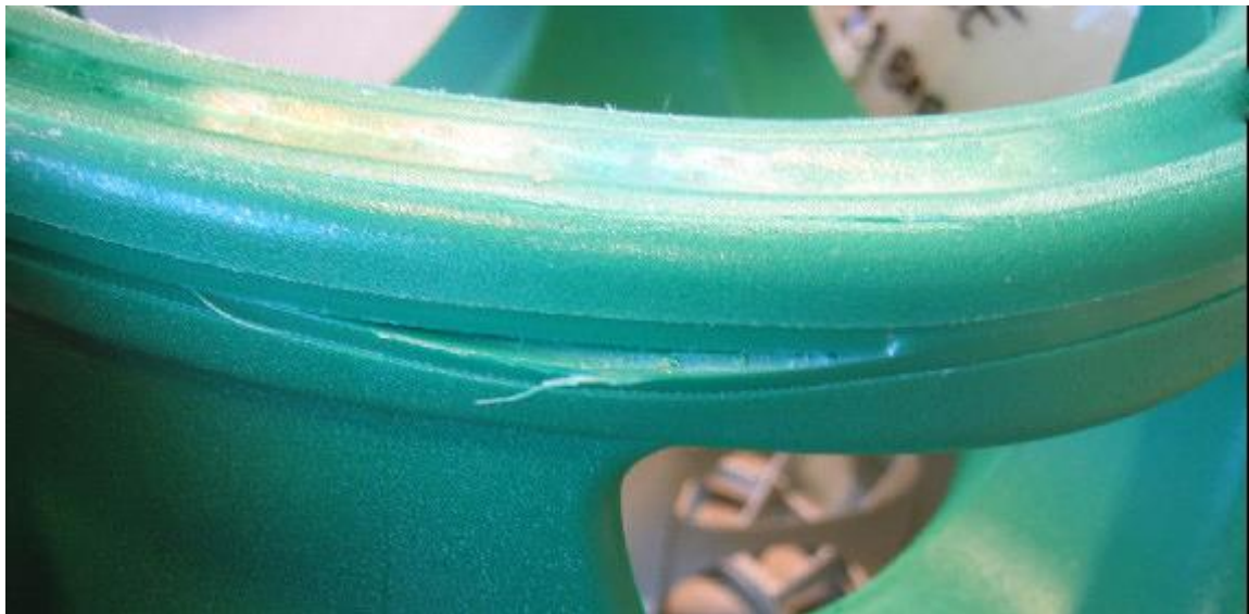
Figures 2 and 3: Unacceptable outer casing damage
